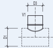
PS/PSU Sattelstück
